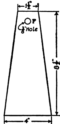
FIG. 75. — Upright.
